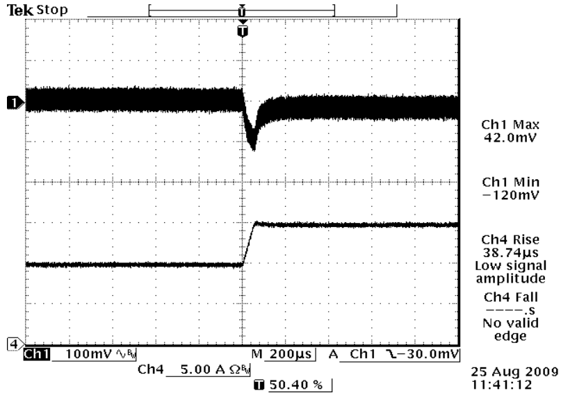
Vout= 5V 50%-75% Load Transients at Vin=48V@Ta=25°C
