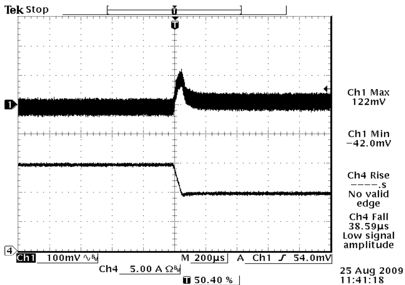
Vout= 5V 75%-50% Load Transients at Vin=48V@Ta=25°C
